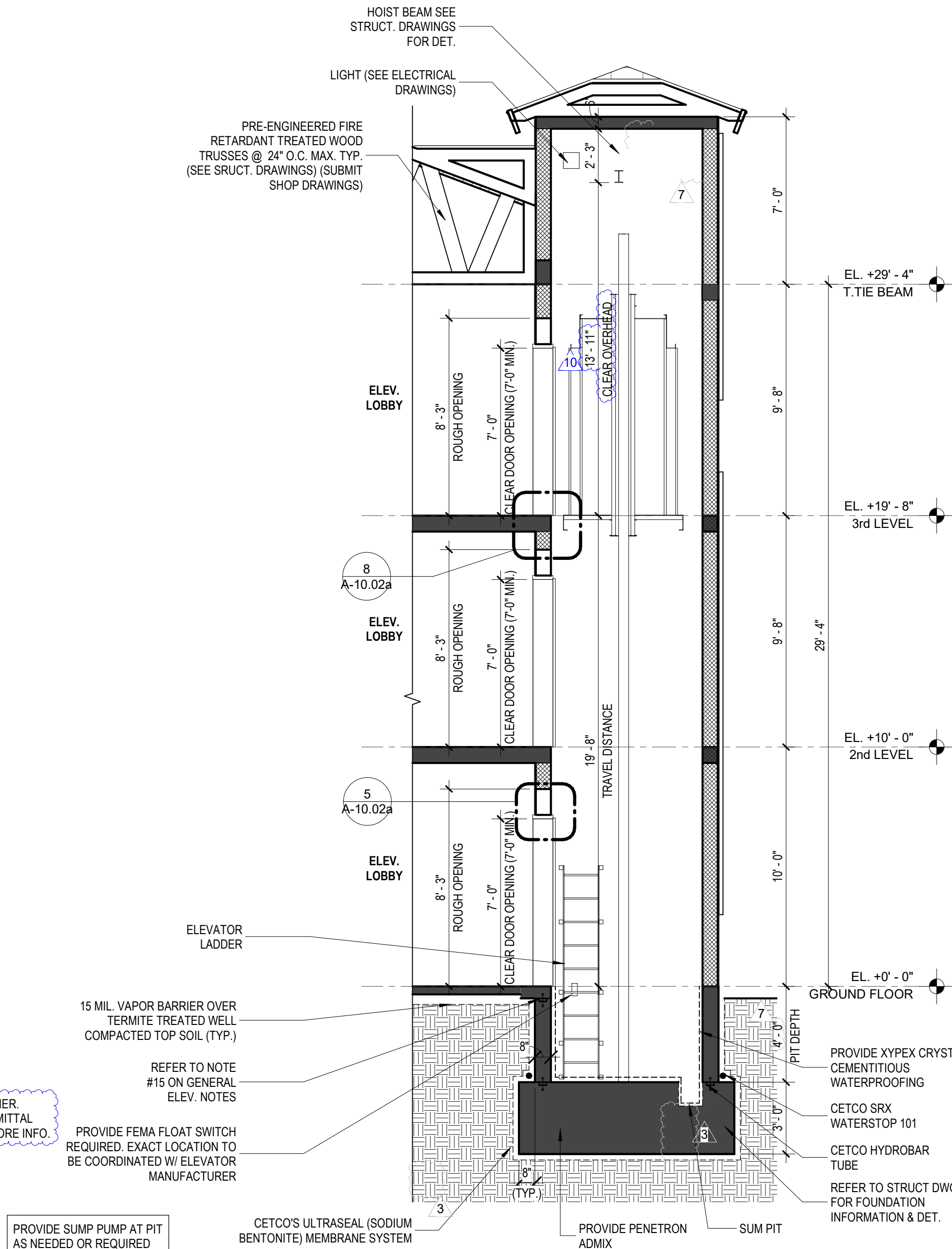
4 BUILDING B - ELEVATOR SECTION SCALE: 1/4" = 1'-0"
