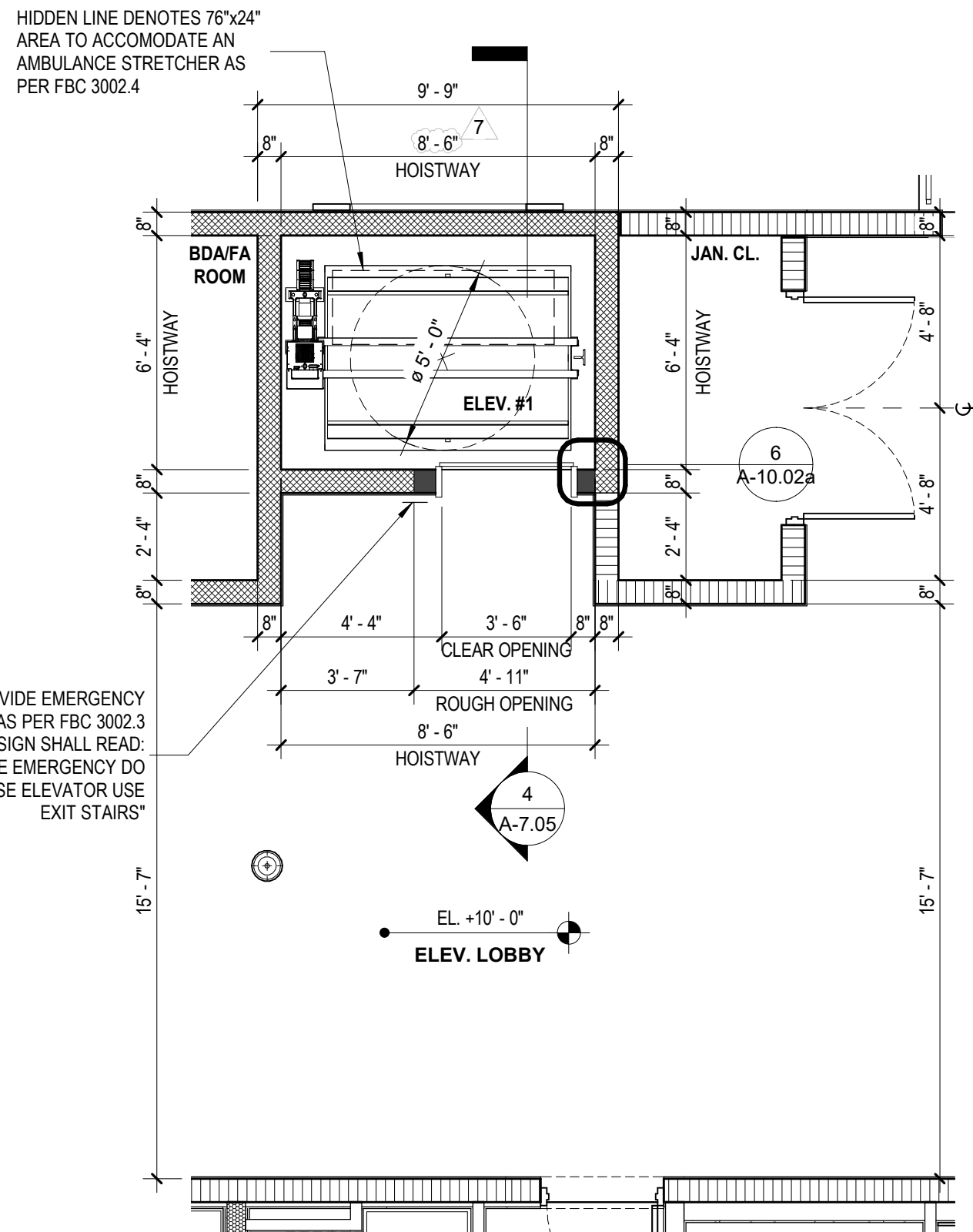
2 BLDG B - ELEV. - 2ND LEVEL SCALE: 1/4" = 1'-0"
