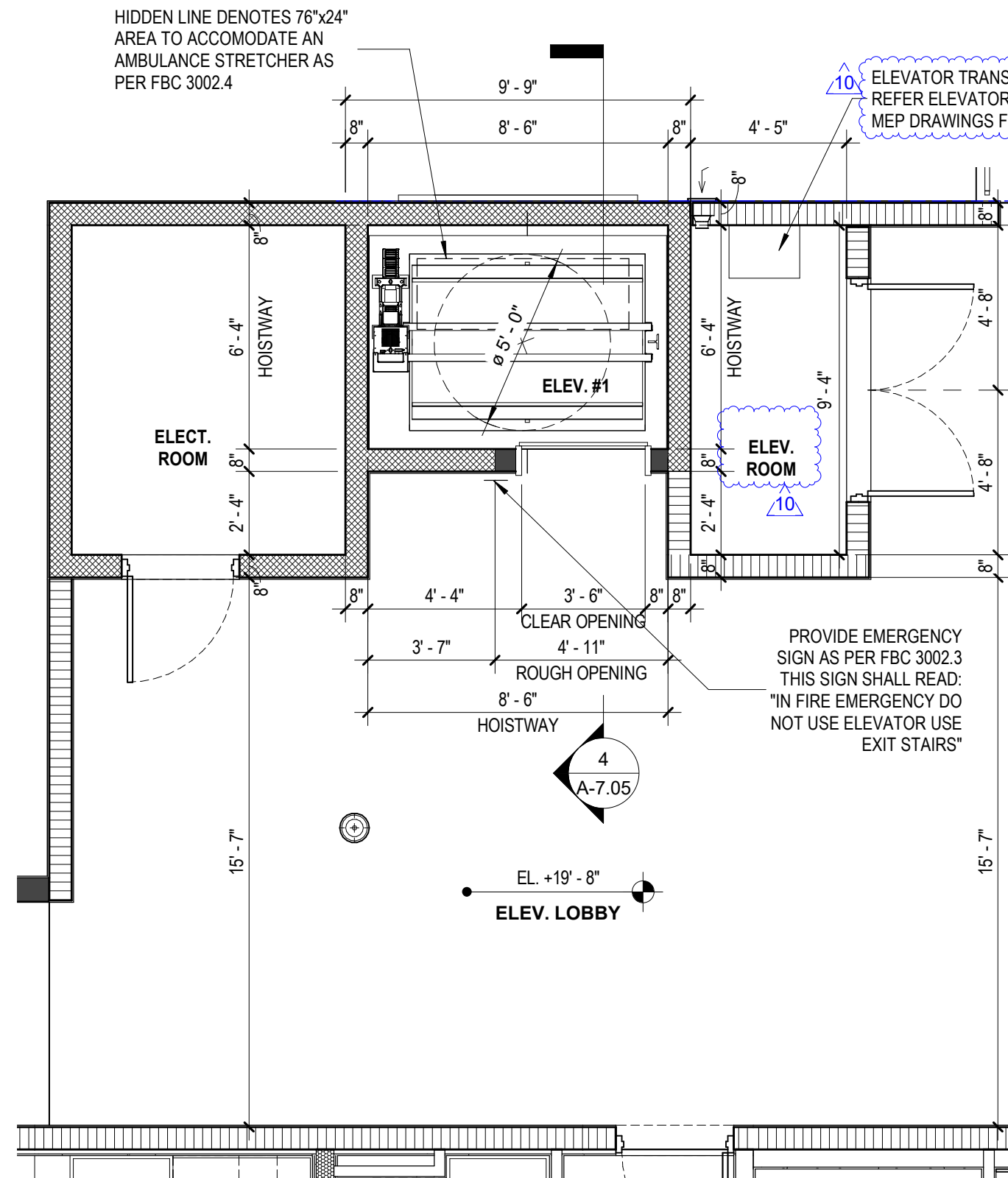
5 BLDG B - ELEV. - 3RD LEVEL SCALE: 1/4" = 1'-0"
