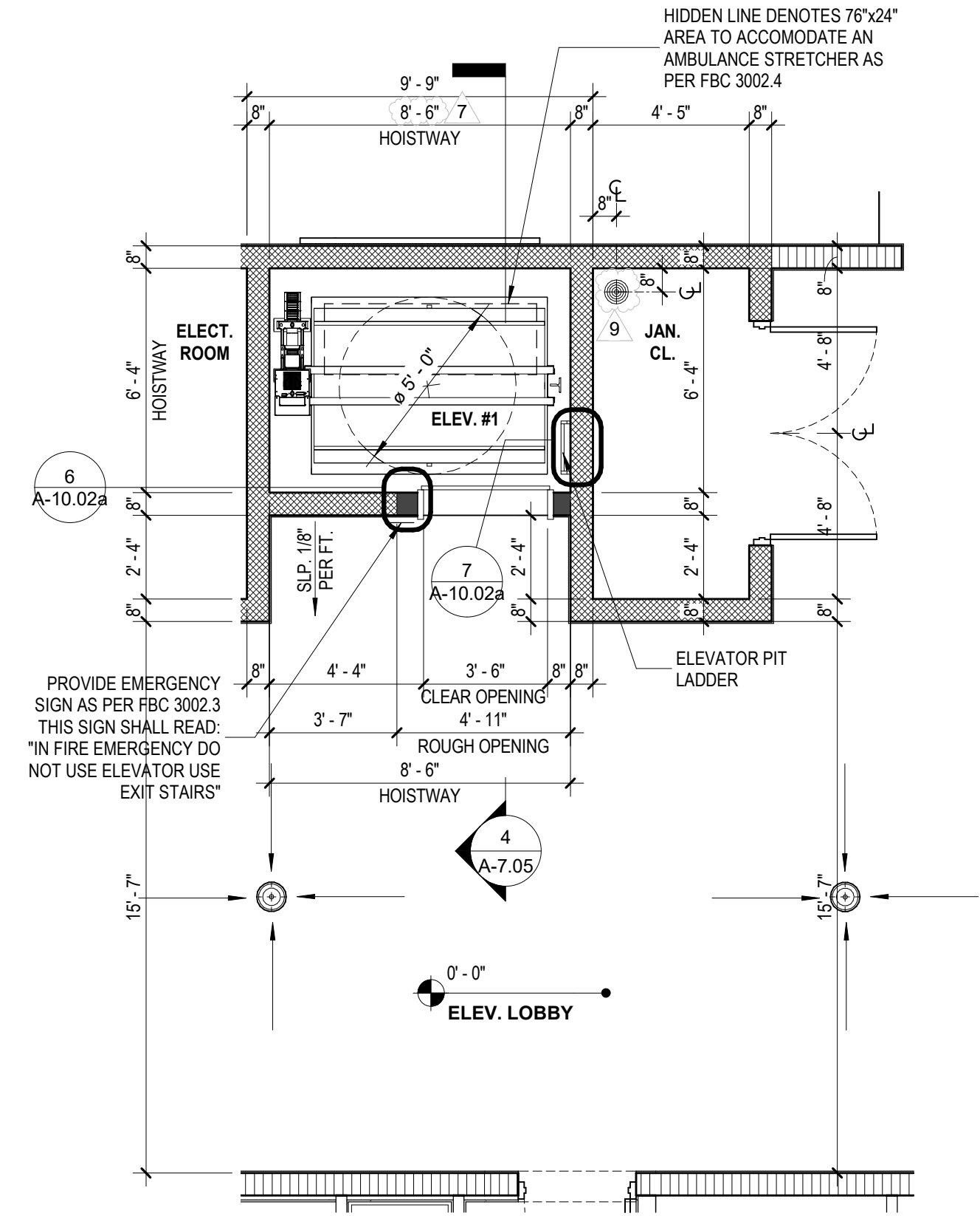
1 BLDG B - ELEV. @ GROUND FLOOR SCALE: 1/4" = 1'-0"
